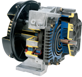
OIL-LESS ROTARY SCROLL (2-5 HP)
