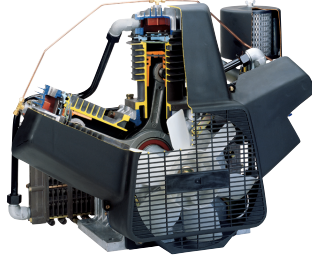
OIL-LESS RECIPROCATING (1-15 HP)
